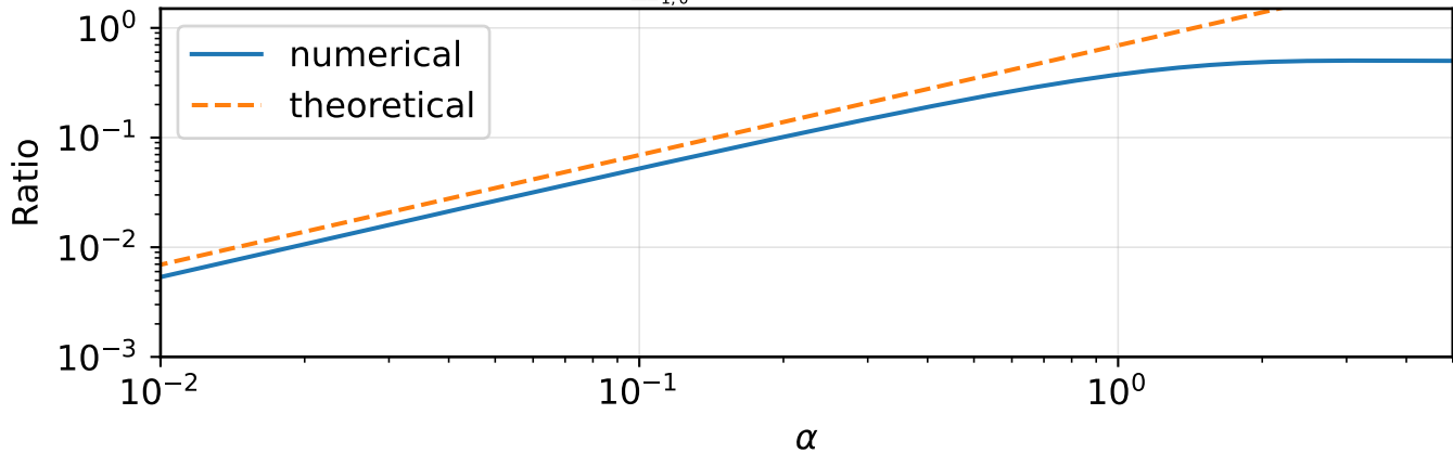
Ratio \frac{\delta E_1}{\Delta E_{1,0}} vs \alpha ( N = 10, J_x = 10.0 )
